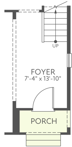
END UNIT CONDITION PORCH SIDE EXTERIOR STYLE C
