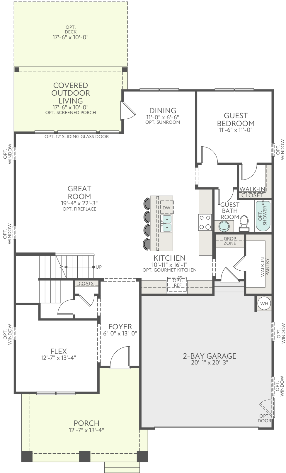
FIRST FLOOR EXTERIOR STYLE B
