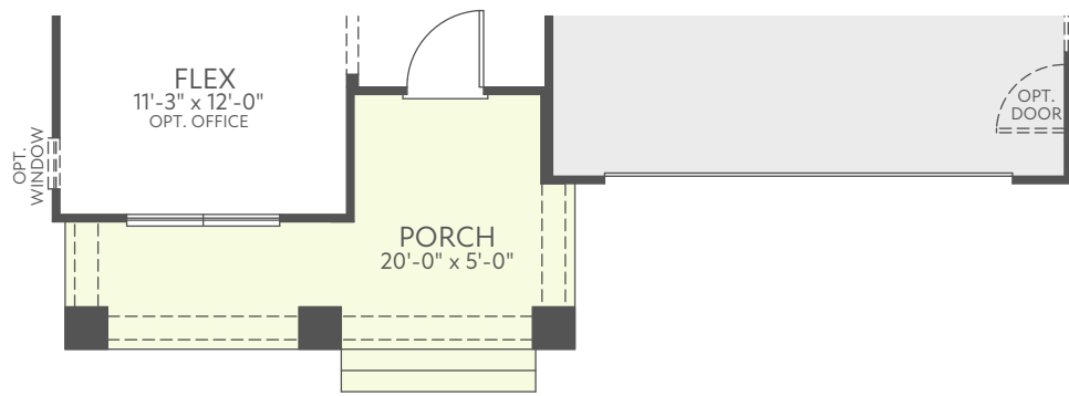
FIRST FLOOR EXTERIOR STYLE B
